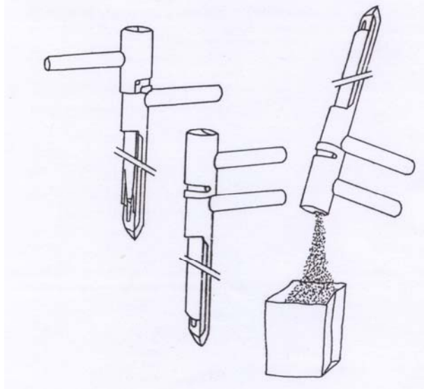
Gambar 2. Alat pengambil contoh model Missouri "D"
